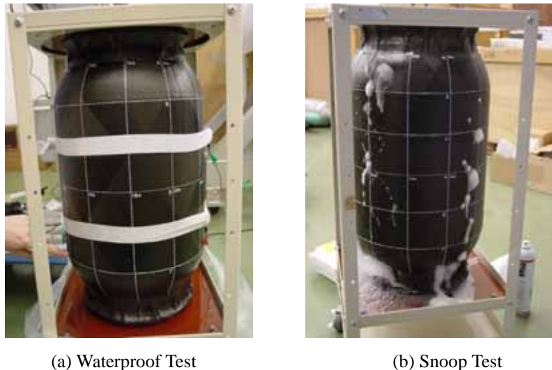
Fig. 21 Waterproof test and snoop test of FW tank.
