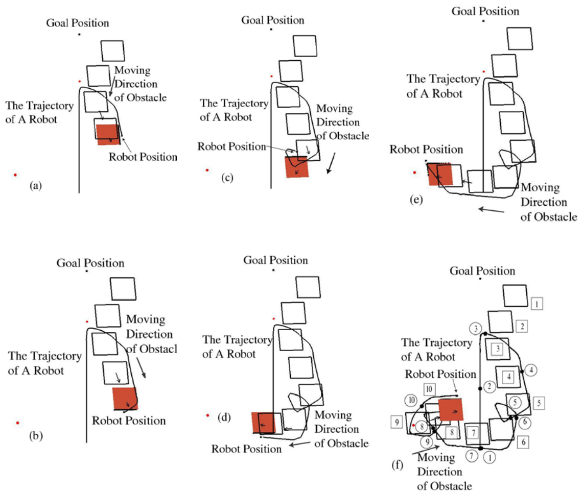
Fig. 6 Failure example for a moving obstacle by T-Bug algorithm.
